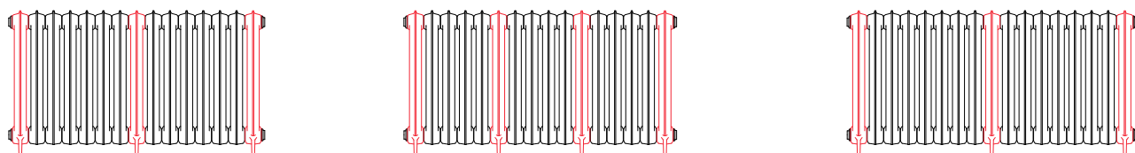
720 x 1262 15 sections (3+12) 720 x 1344 16 sections (4+12) 720 x 1426 17 sections (3+14)
