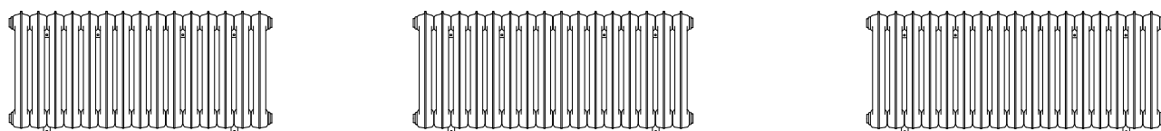
560 x 1262 15 sections 560 x 1344 16 sections 560 x 1426 17 sections
