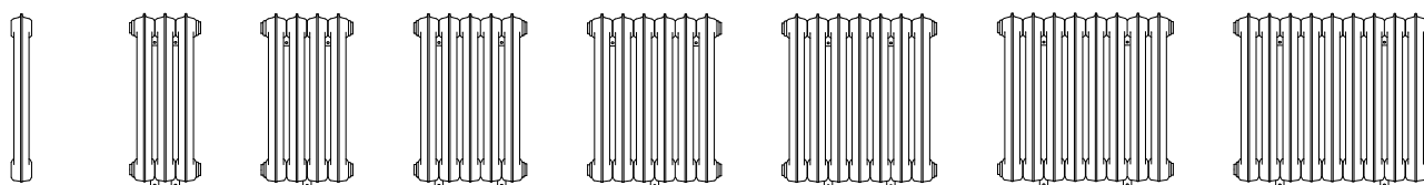
660 x 80 1 section 660 x 278 3 sections 660 x 360 4 sections 660 x 442 5 sections 660 x 524 6 sections 660 x 606 7 sections 660 x 688 8 sections 660 x 770 9 sections
